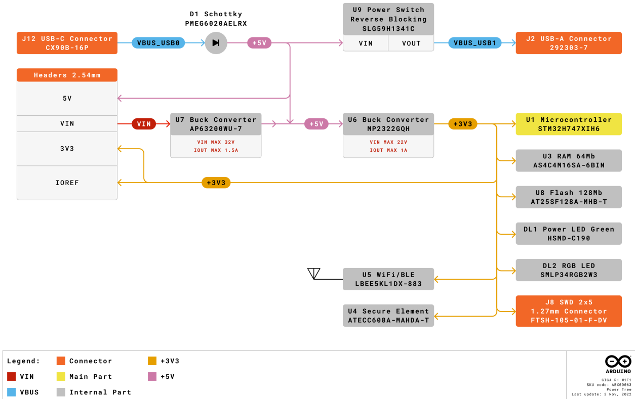
Arduino GIGA R1 WiFi Power Tree
