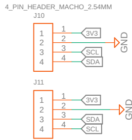
4_PIN_HEADER_MACHO_2.54MM
