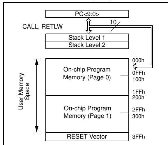
FIGURE 6-2: PIC16C56/CR56 PROGRAM MEMORY MAP AND STACK
