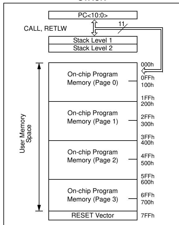
FIGURE 6-3: PIC16C57/CR57/C58/CR58 PROGRAM MEMORY MAP AND STACK
